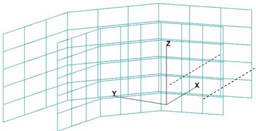
Figure 44: The cylindrical test target.
