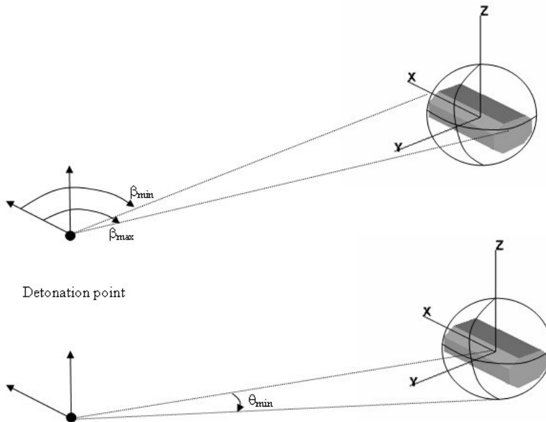
Figure 7 Limitations for bearing and elevation for fragment selection.
