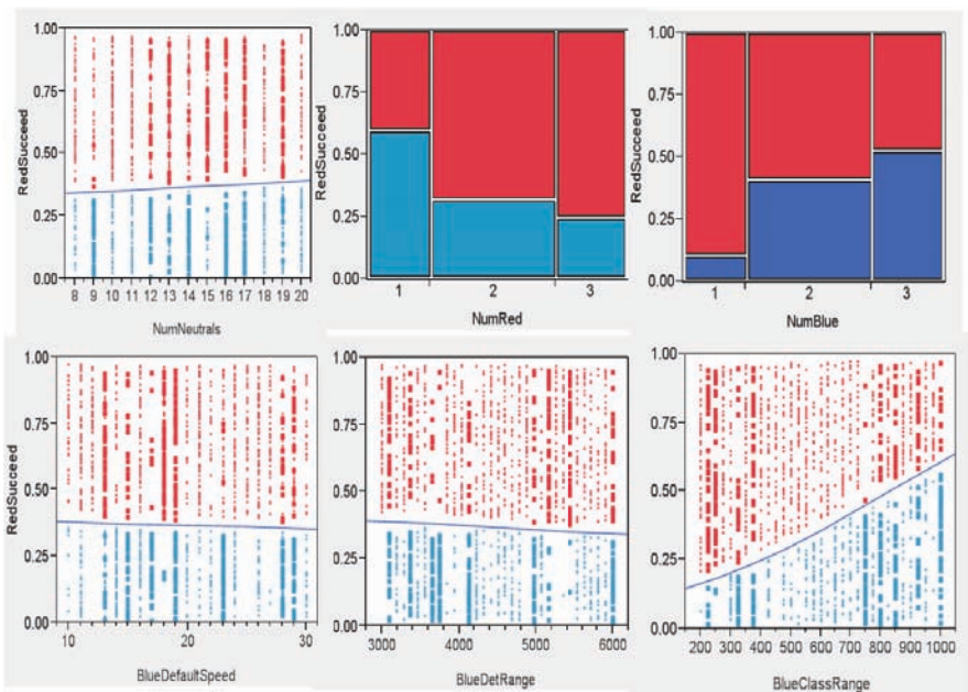
Figure 3: Partition Tree and Logistic Fit
