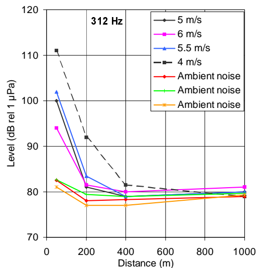
Figure 11. Same as Figure 10 but for the frequency 312 Hz.
