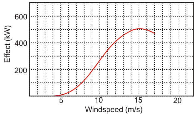
Figure 7. Effective output for Wind World 500 kW, depending on wind speed.
