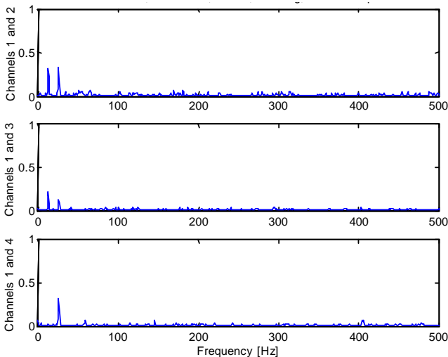
Figure 12. The mean coherence between the hydrophones, calculated from a background noise measurement. Upper; the coherence between hydrophone 1 and 2, (50 m and 200 m). Middle; the coherence between hydrophone 1 and 3, (50 m and 400 m). Lower; the coherence between hydrophone 1 and 4, (50 m and 1000 m).
