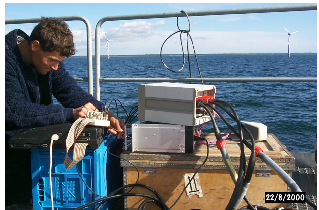
Figure 3. The four hydrophones were simultaneously recorded with the sampling equipment placed outside on the working platform at Bockstigen 1. The wind mills Bockstigen 2 and 3 can be seen in the background.
