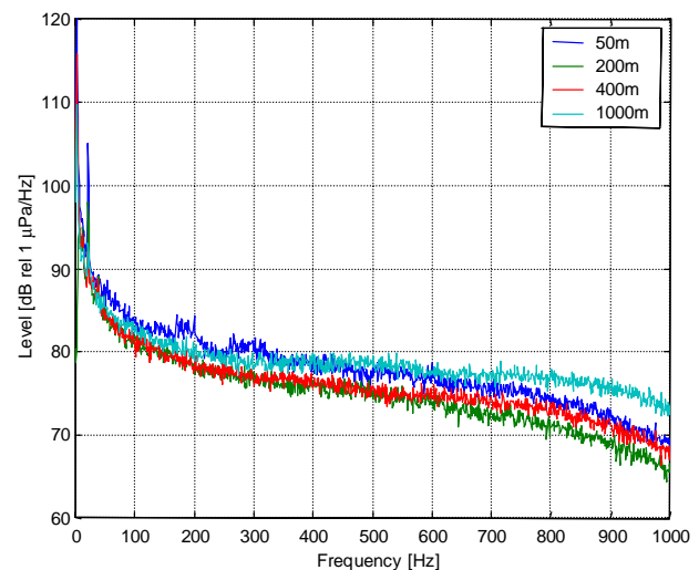
Figure 8. Spectral levels at the distances 50, 200, 400 and 1000 m (different colours) from Bockstigen 1 when the mill is stopped. The wind speed is 4 – 5 m/s, (similar to Figure 6).
