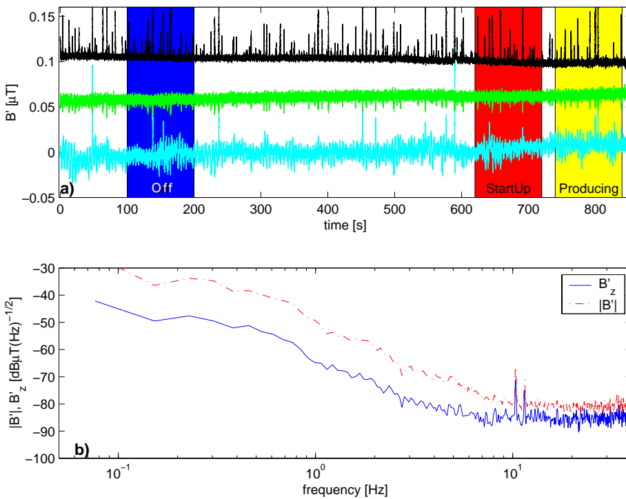
Figure 16. 900 s recording of the 24 dB-amplified part of the magnetic field during halt-, startup- and producing-periods at the location Magpos1 (400 m).
