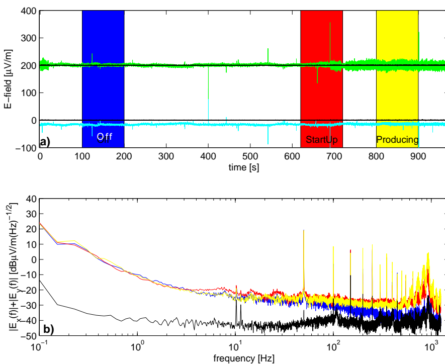
Figure 17. 1000 s recording of the horizontal electrical field during halt-, startup- and producing-periods at the location Elpos2 (144 m).
