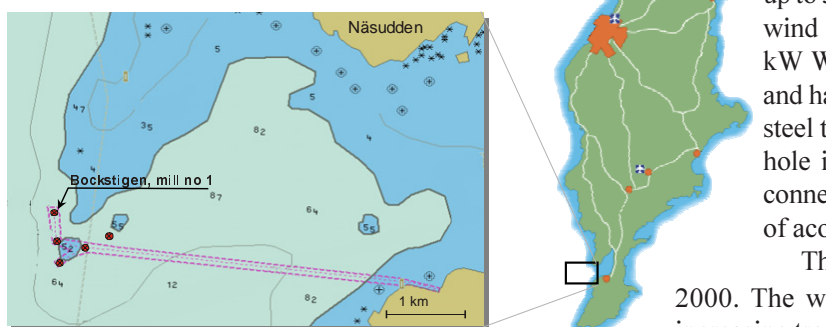
Figure 1. Bockstigen offshore wind mill park is located 4 – 5 km southwest from the Näsudden peninsula on Gotland. The measurements were carried out west of Bockstigen number 1. Indicated in the map is also the power cable connection to the mainland, (the red dotted lines).
