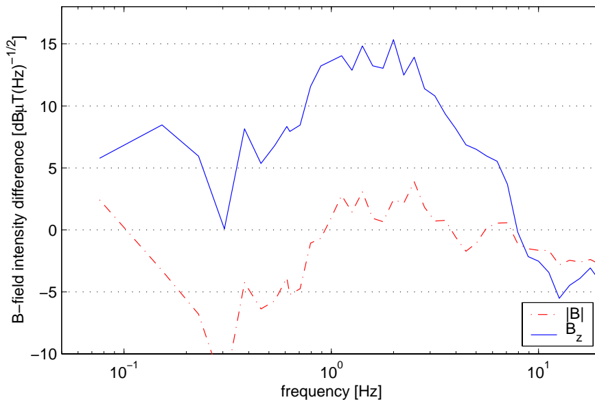
Figure 20. Difference between the energy content of the vertical component of the magnetic field B'_z and the sum of the absolute value of all three components in the frequency domain at the two locations Magpos1 and Magpos2.
