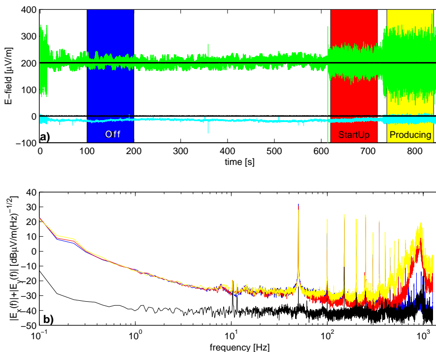
Figure 15. 900 s recording of the horizontal electrical field during halt-, startup- and producing-periods at location Elpos1 (366 m).
