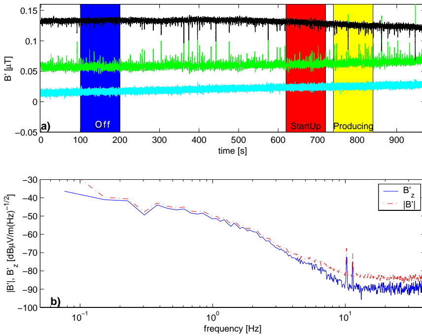
Figure 19. 1000 s recording of the 24 dB-amplified part of the magnetic field during halt-, startup- and producing-periods at the location Magpos2 (209 m). a) Time series where the three stages are marked by different colour. The three curves are denoted (from the bottom of the panel) B'_x , B'_y and B'_z respectively. b) Spectral representation of the vertical component of the magnetic field B'_z and the sum of the absolute value of all three components in the frequency domain, i.e. |B'_x(f)| + |B'_y(f)| + |B'_z(f)| .
