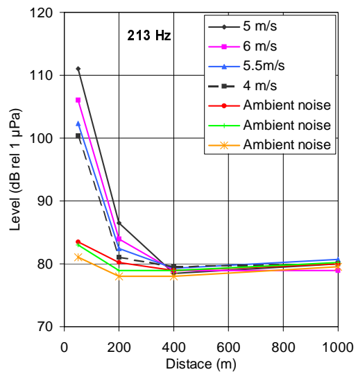
Figure 10. Comparison between seven different data sets for the spectral levels at 213 Hz. Three of these measurements were carried out when the mill Bockstigen 1 was stopped, (ambient noise). The wind speed was in the range 4 – 6 m/s in all seven cases.
