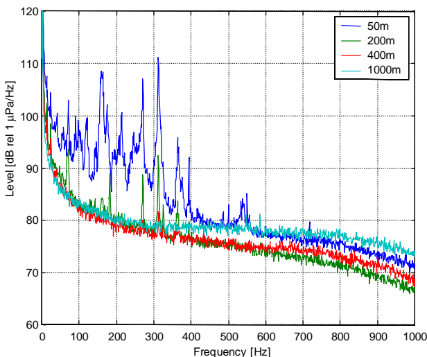
Figure 6. Spectral levels at the distances 50, 200, 400 and 1000 m (different colours) from Bockstigen 1. The mill is here rotating in a light wind at 4 – 5 m/s.
