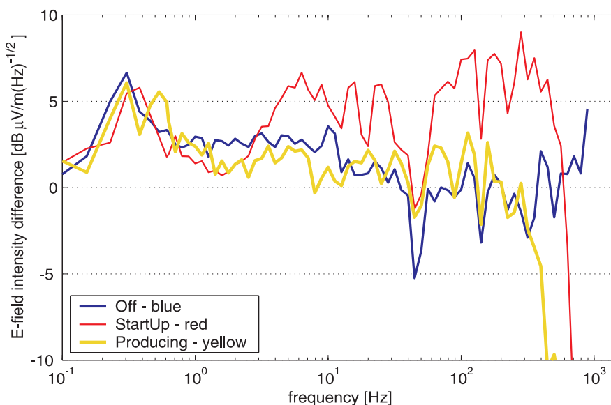
Figure 18. Difference between the energy content of the horizontal components of the electrical field at the two locations, Elpos1 and Elpos2, as a function of frequency. The three stages (Off, startup and producing) are colour coded according to Figure 15-17.
