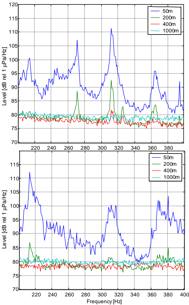
Figure 9. Spectral levels in the frequency range 200 – 400 Hz from two occasions during the measuring period, August 22 (upper) and August 23 (lower). The wind conditions were similar, 4 – 5 m/s blowing from 268 - 286°.
