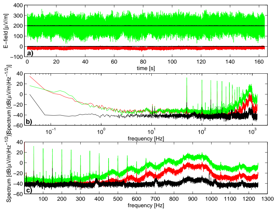
Figure 13. 160 s recording of the electrical field at location Elpos1 (366 m).
