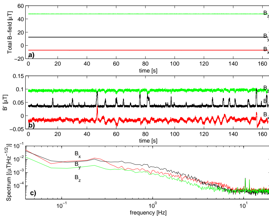
Figure 14. 160 s recording of the magnetic field at location, Magpos1 (400 m).
