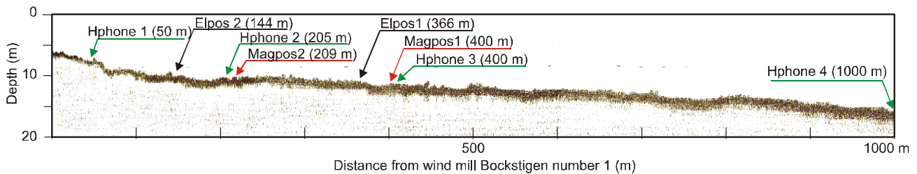
Figure 2. The bottom profile at the studied area, outside mill number 1 at Bockstigen. The positions of the sensors are indicated, where Hphone 1-4 are the four hydrophones. Elpos 1, 2 are the two positions of the electrode and Magpos 1, 2 are the two positions of the magnetometer.
