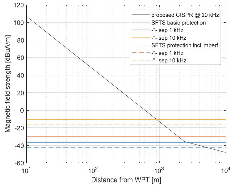
Figure 5.1: WPT emission level at 20 kHz, compared to protection criteria for SFTS.
