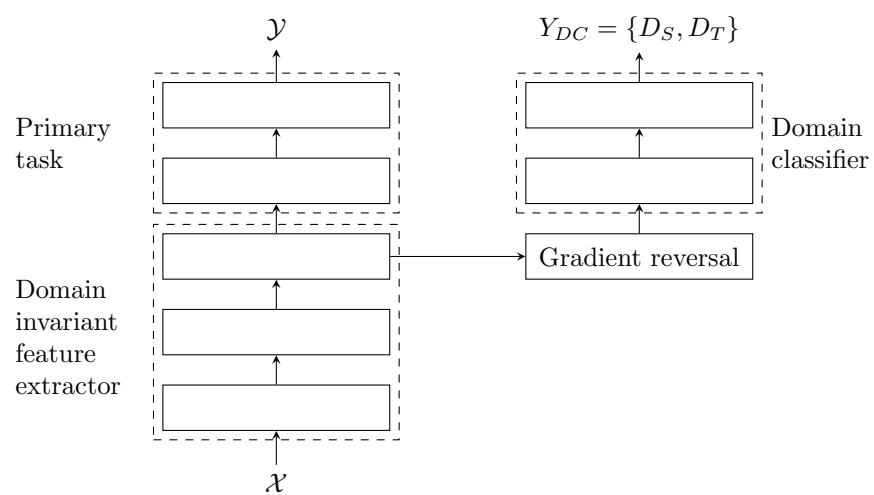
Figure 3.2: UDA using an adversarial multi-task learning approach [58].
