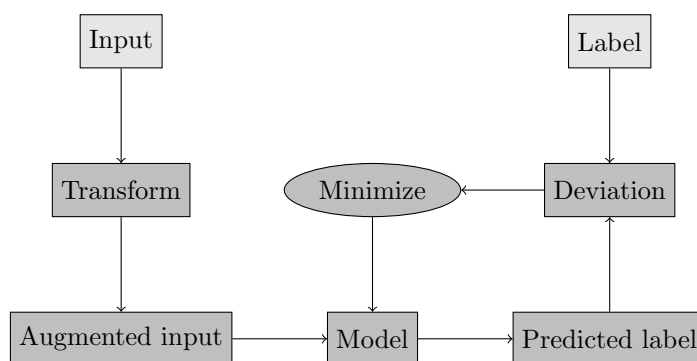
Figure 2.1: Data augmentation in supervised learning. Learning is performed using inputs that have been augmented using various transformation functions. Light gray boxes represent training data (i.e., inputs and their labels).
