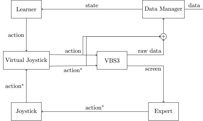
Figure 4.2: Illustration of control and data gathering setup. The star superscript marks the expert (human) pilot.
