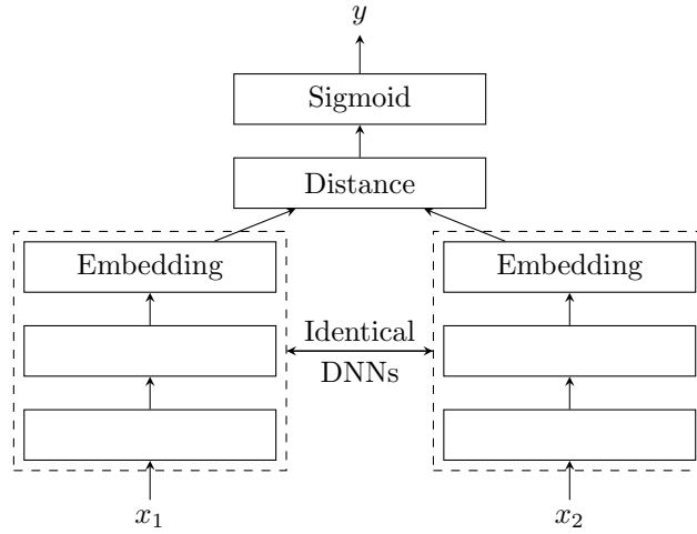
Figure 3.6: Siamese networks consist of two identical networks that share a single head. The network is capable of calculating a similarity metric given an input pair. Each input is first processed by the twin networks to generate an embedding. The embedding is then merged into a single head using a distance layer whose output is then processed by an output layer where a sigmoid activation function is used to produce a similarity value that can be thresholded to determine if the two inputs are from the same class or not. Siamese networks can be trained using binary cross-entropy, contrastive or triplet loss functions.
