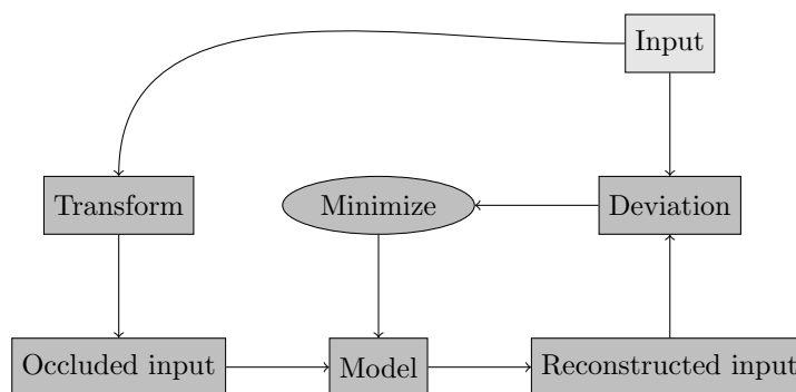
Figure 2.3: Similar to supervised learning, the objective of the self-supervised learning process is to create a model that minimizes the deviation from the presented training examples. In this case the task is to learn how to reconstruct (automatically created) occluded versions of the original inputs.
