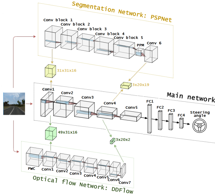
Figure 3.4: A DNN is trained to predict steering wheel angle of a self-driving car using images, where a segmentation network and an optical flow network contribute with their extracted features with soft parameter sharing. The two auxiliary networks are discarded after training [71].
