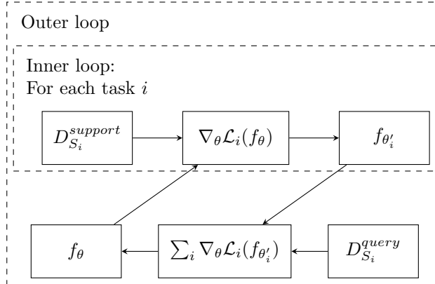
Figure 3.5: MAML consists of two loops. The inner loop learns specific tasks using a support dataset, D_{S_i}^{support} , that consists of only k training examples (or k \times n in the classification case) to promote fast adaptation. The outer loop then uses a query dataset, D_{S_i}^{query} , and the information gained in the inner loop (i.e., \theta'_i ) to update the trainable parameters in \theta . The outer loop updates \theta so that the meta-objective, in this case the average performance over all tasks, is increased.
