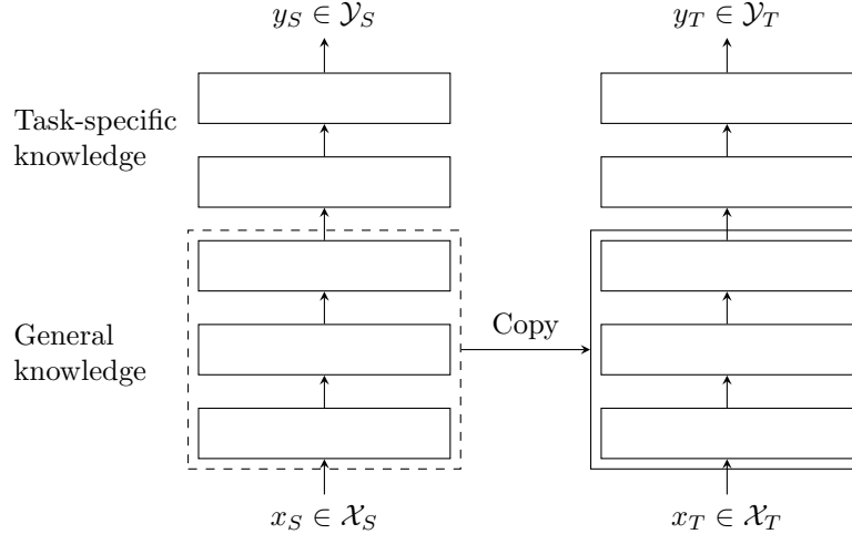
Figure 3.1: Pre-training and fine-tuning is performed by copying layers from a source model (left) to a target model (right). Only the task-specific layers closest to the output in the target model need to be trained. When successfully applied the target training data, D_T , is typically much smaller than the source training data, D_S .
