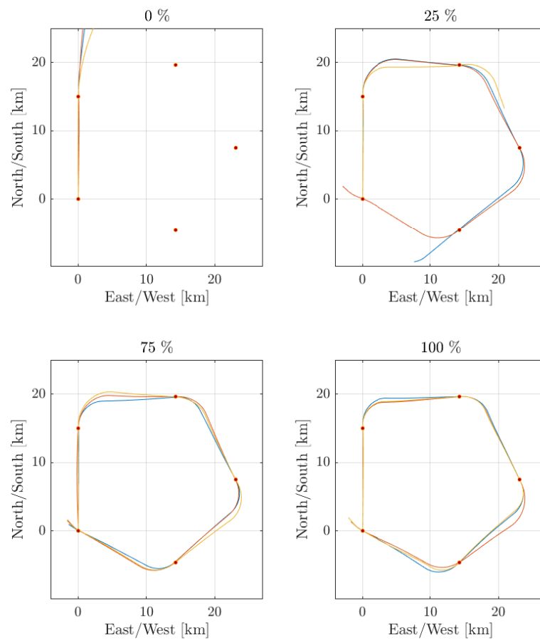
Figure 4.3: Learning process for Policy B: Plots showing the resulting trajectories for different amounts of data used in training. The red dots are spheres of radius 250 m , which indicates the error margin.
